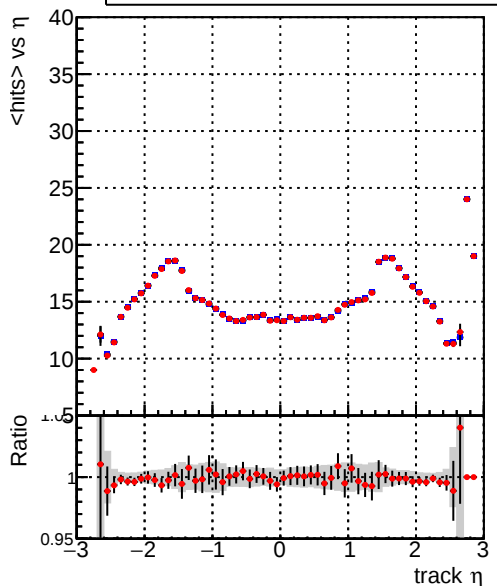
mean hits vs \eta Legend: DQM_mkFit_TT_base (blue line), DQM_mkFit_TT_retrain (red line)
