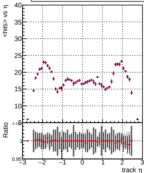
mean hit — DQM_mkFit_TT_base — DQM_mkFit_TT_retrain
