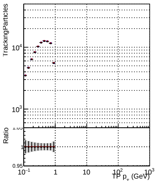
Legend: - DQM_mkFit_TT_base (blue circles) - DQM_mkFit_TT_retrain (red circles) - DQM_mkFit_TT_retrain_noCandDNN (black circles)
