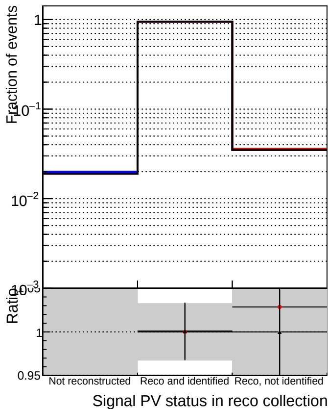
—■ DQM_mkFit_TT_base —● DQM_mkFit_TT_retrain —● DQM_mkFit_TT_retrain_noCandDNN
