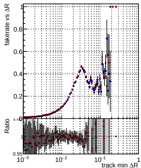
Legend for all plots: DQM_mkFit_TT_base (Blue circles) DQM_mkFit_TT_retrain (Red circles) DQM_mkFit_TT_retrain_noCandDNN (Black circles)
