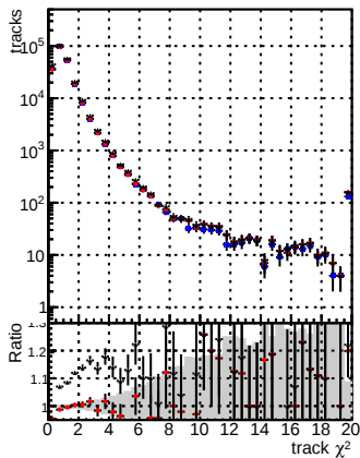
DQM mkFit || base DQM mkFit || retrain N of reco track vs. s DQM mkFit || retrain noCandDNN
