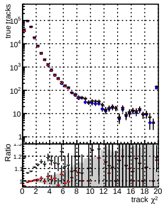
noCandDNN
