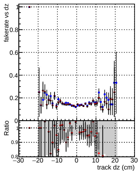
—●— DOM mkFit TT base —●— DOM mkFit TT retrain —●— noCandDNN
