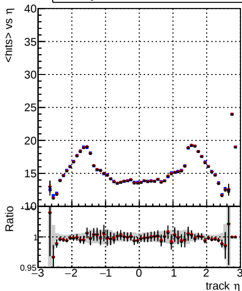
mean hits vs \eta — DQM_mkFit_TT_base — DQM_mkFit_TT_retrain — DQM_mkFit_TT_retrain_noCandDNN
