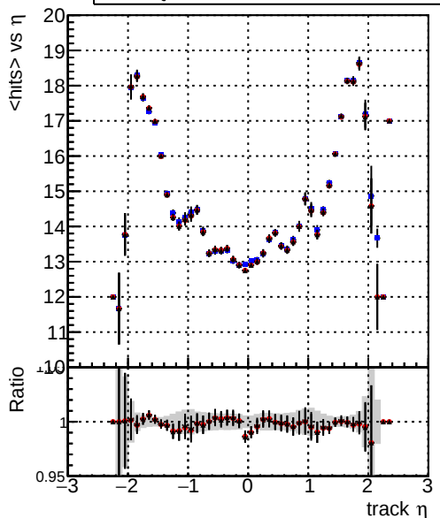
mean hits vs \eta — DQM_mkFit_TT_base — DQM_mkFit_TT_retrain — DQM_mkFit_TT_retrain_noCandDNN
