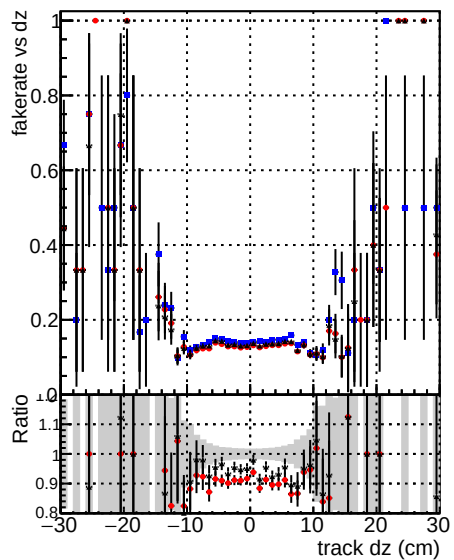
— DOM mkFit TT base — retrain — DOM mkFit TT retrain noCandDNN
