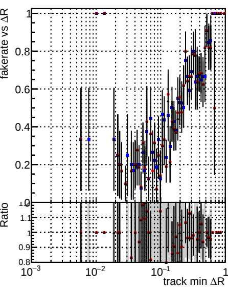
Legend: DQM_mkFit_TT_base (blue dots), DQM_mkFit_TT_retrain (red dots), DQM_mkFit_TT_retrain_noCandDNN (black dots)
