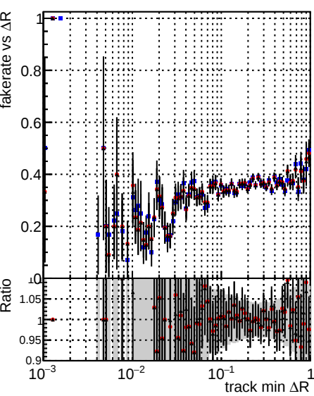
Legend: DQM_mkFit_TT_base (blue circles), DQM_mkFit_TT_retrain (red circles), DQM_mkFit_TT_retrain_noCandDNN (black circles)
