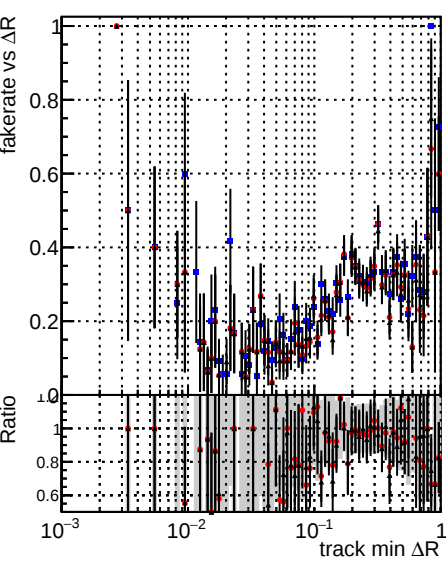
Fake rate vs \Delta R(\text{track, jet}) Legend: DQM_mkFit_TT_base (blue stars) DQM_mkFit_TT_retrain (red stars) DQM_mkFit_TT_retrain_noCandDNN (black stars)
