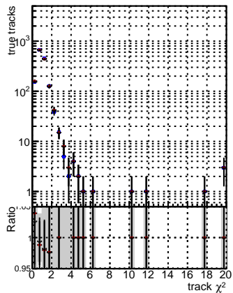
noCandDNN
