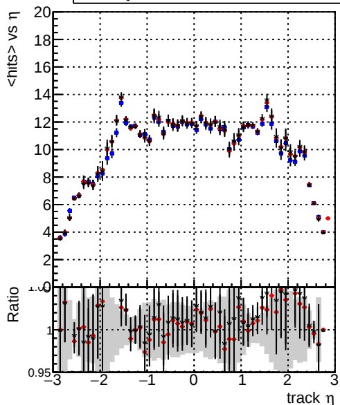
mean hits vs \eta — DQM_mkFit_TT_base — DQM_mkFit_TT_retrain — DQM_mkFit_TT_retrain_noCandDNN
