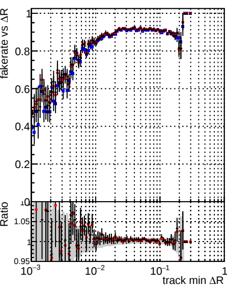
Fake rate vs \Delta R (track, jet) DQM_mkFit_TT_base DQM_mkFit_TT_retrain DQM_mkFit_TT_retrain_noCandDNN
