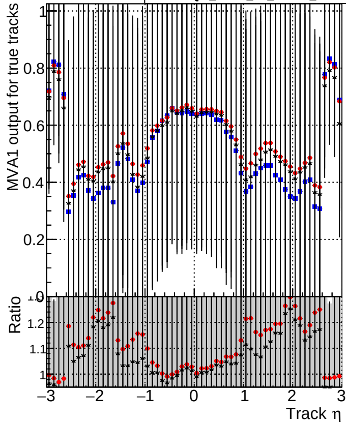
MVA1 of associated tracks (recoToSim) vs. track \eta Legend: —■— DQM_mkFit_TT_base —●— DQM_mkFit_TT_retrain —▲— DQM_mkFit_TT_retrain_noCandDNN
