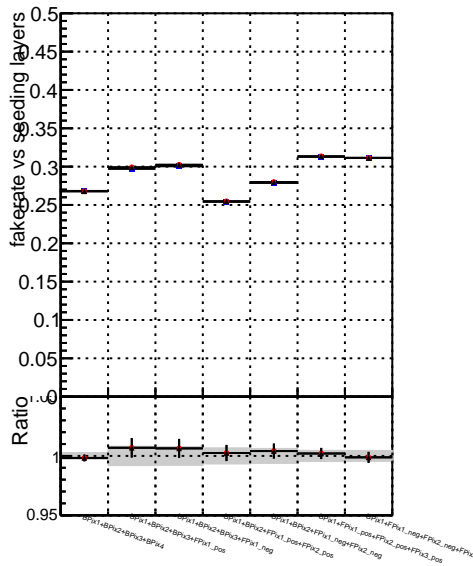
Fake rate vs. ■ DGM ● mkFit ▲ TT base ◆ retrain ■ DGM ● mkFit ▲ TT retrain noCandDNN
