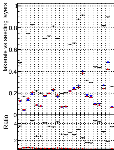
DOM mkFit TT base DOM mkFit TT retrain DOM mkFit TT retrain noCandDNN
