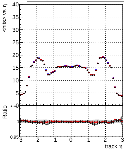
mean hit Legend: DQM_mkFit_TT_base DQM_mkFit_TT_retrain DQM_mkFit_TT_retrain_noCandDNN
