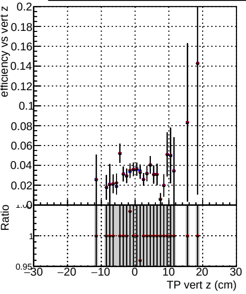
Efficiency vs vertpos DQM_mkFit_TT_base DQM_mkFit_TT_retrain DQM_mkFit_TT_retrain_noCandDNN
