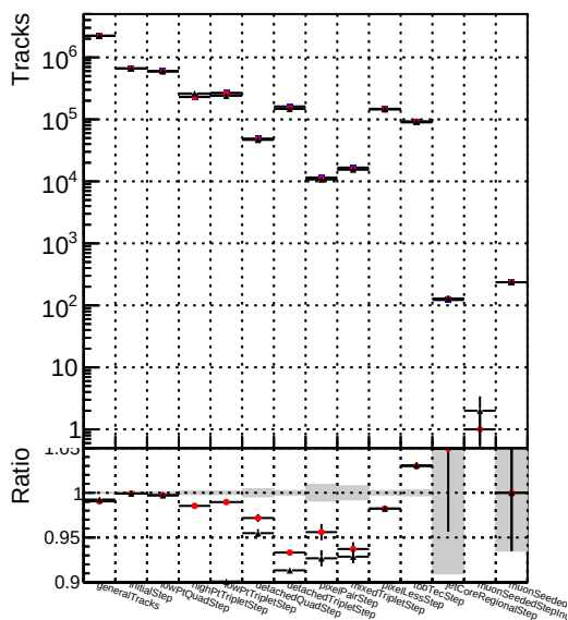
Number of tracks vs collection Legend: DQM_mkFit_TT_base (blue circles) DQM_mkFit_TT_retrain (red circles) DQM_mkFit_TT_retrain_noCandDNN (black circles)
