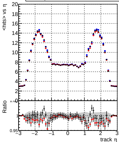
— DQM_mkFit_TT_base — DQM_mkFit_TT_retrain — DQM_mkFit_TT_retrain_noCandDNN mean hit
