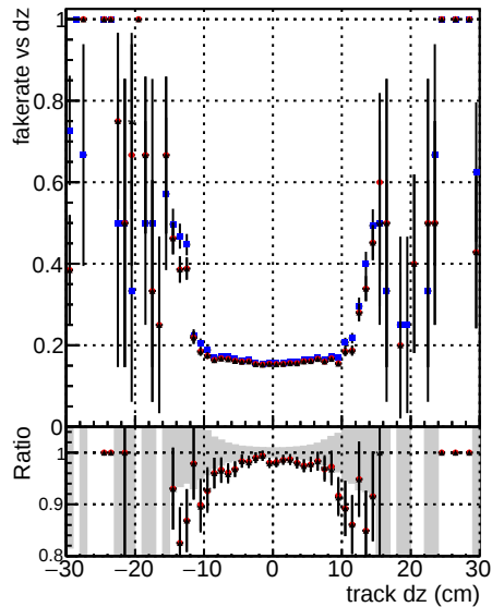
— DOM mkFit TT base — DOM mkFit TT retrain — DOM mkFit TT retrain noCand — DNN
