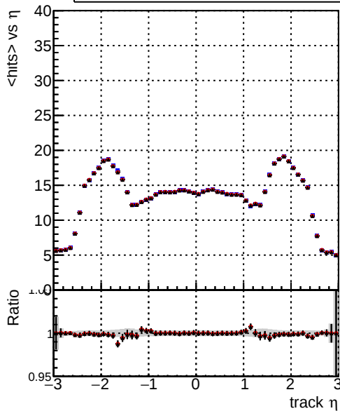
— DQM_mkFit_TT_base — DQM_mkFit_TT_retrain — DQM_mkFit_TT_retrain_noCandDNN mean hit
