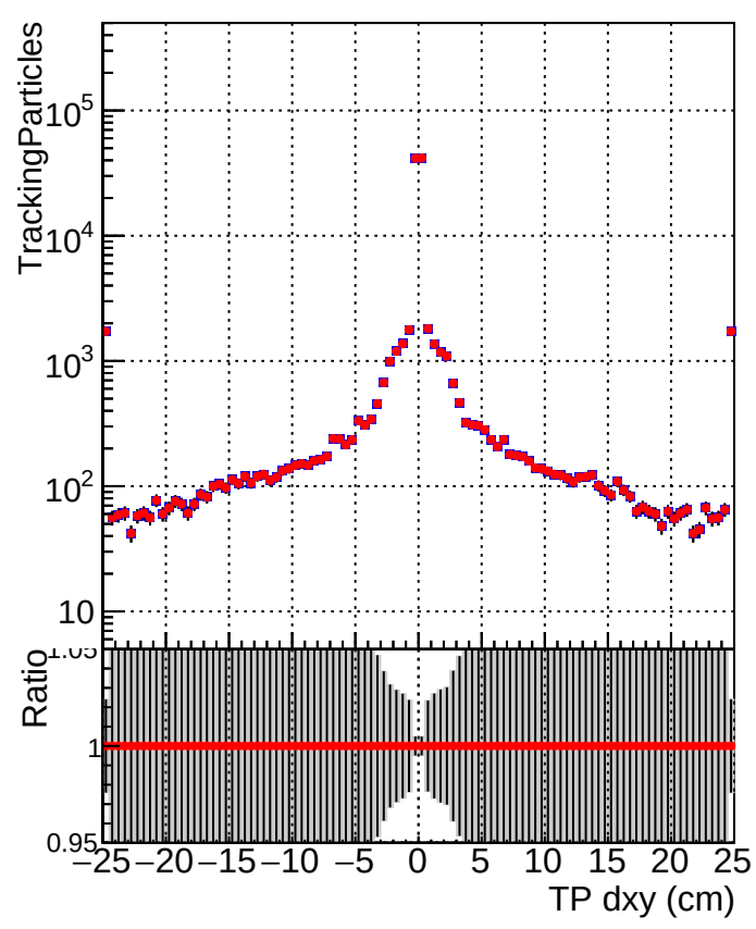
N of simulated track Legend: ■ DQM_CKF_TT_base ● DQM_CKF_TT_retrain
