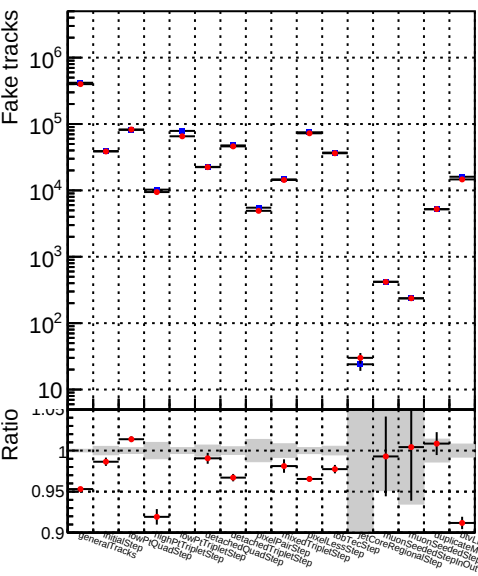
Number —●— DQM_CKF_TT_retrain
