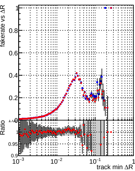
Fake rate vs \Delta R (track, jet) DQM_CKF_TT_base DQM_CKF_TT_retrain
