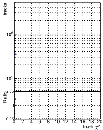
N of reco track vs. \chi^2 (base vs. retrain)
