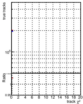
N of associated (recoToSim) tracks vs. \chi^2 (base vs. retrain)
