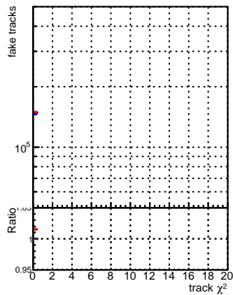
N of fake tracks vs. \chi^2 (base vs. retrain)
