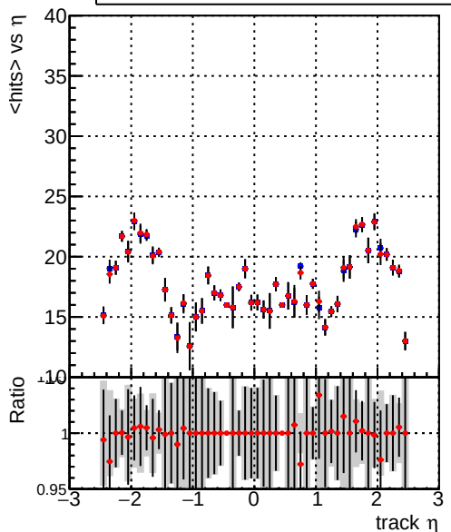
mean hit — DQM_CKF_TT_base — DQM_CKF_TT_retrain
