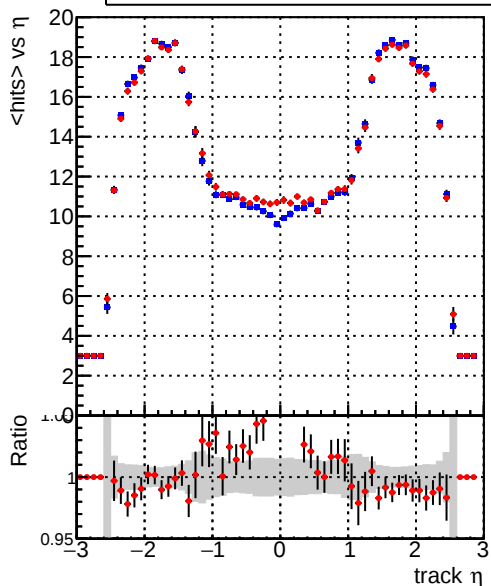
mean hits vs \eta — DQM_CKF_TT_base — DQM_CKF_TT_retrain
