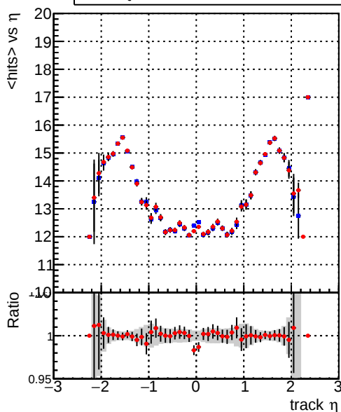
mean hits vs \eta Legend: DQM_CKF_TT_base (blue line), DQM_CKF_TT_retrain (red line)
