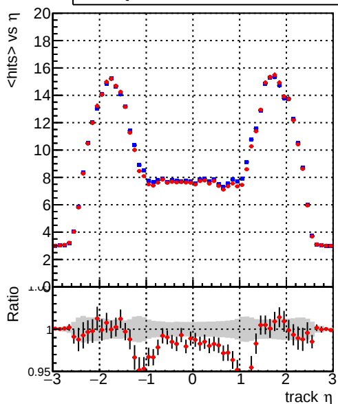
mean hit — DQM_CKF_TT_base — DQM_CKF_TT_retrain
