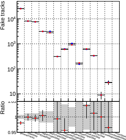
Number —●— DQM_CKF_TT_retrain
