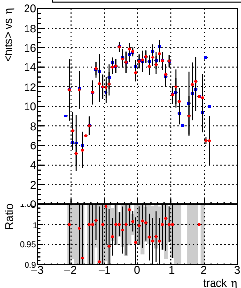
mean hit Legend: DQM_CKF_TT_base (blue line), DQM_CKF_TT_retrain (red line)
