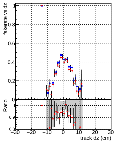
Fake rate vs dz —●— DQM_CKF_TT_base —●— DQM_CKF_TT_retrain
