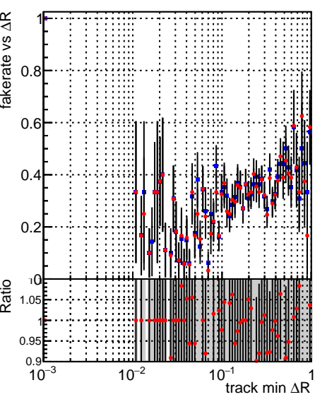
Fake rate vs \Delta R(\text{track, jet}) ◆ DQM_CKF_TT_base ● DQM_CKF_TT_retrain
