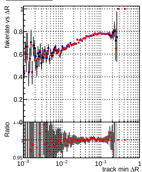
Fake rate vs DQM_CKF_TT_base DQM_CKF_TT_retrain
