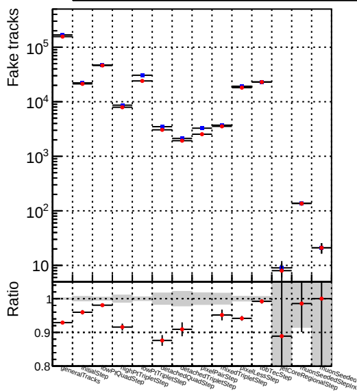
Number —●— DQM_CKF_TT_retrain
