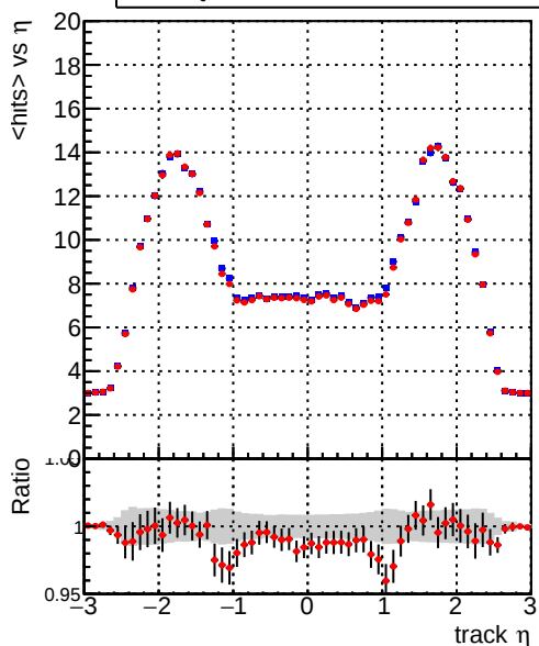
mean hits vs \eta — DQM_CKF_TT_base — DQM_CKF_TT_retrain
