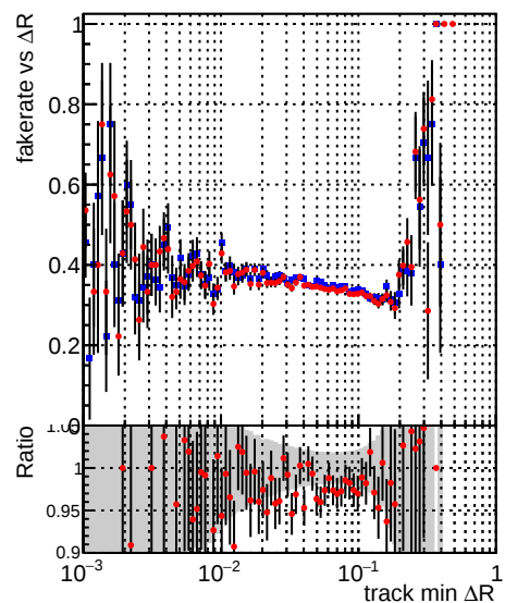
—•— DQM_CKF_TT_base —•— DQM_CKF_TT_retrain
