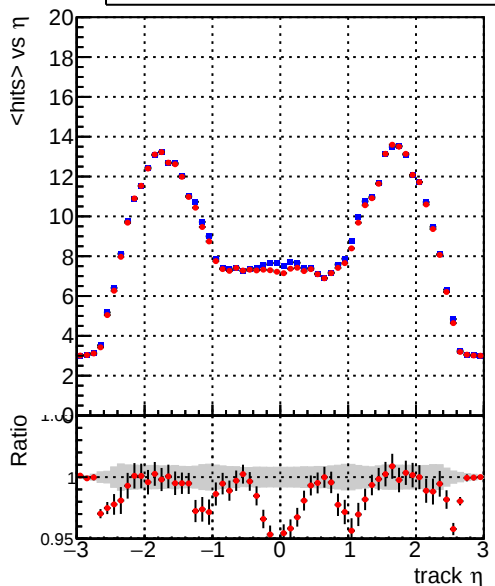
mean hits vs \eta — DQM_CKF_TT_base — DQM_CKF_TT_retrain
