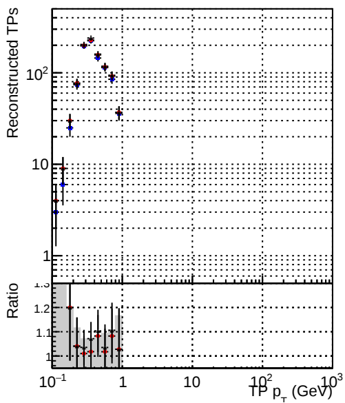
Legend: DQM_mkFit_TT_base (Blue circles) DQM_mkFit_TT_retrain_noCandDNN (Red circles) DQM_mkFit_TT_retrain (Black circles)
