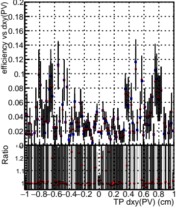
Efficiency vs Dxy(PV) legend: DQM_mkFit_TT_base, DQM_mkFit_TT_retrain_noCandDNN, DQM_mkFit_TT_retrain
