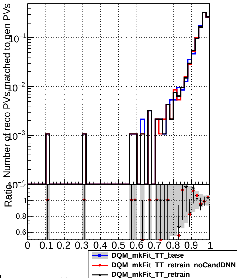
RecoPVAssoc2GenPVmatched_missing
