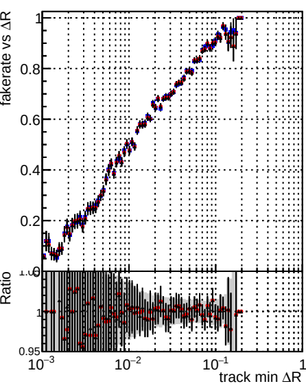
Fake rate vs \Delta R(\text{track, jet}) Legend: DOM mkFit TT base DOM mkFit TT retrain_noCandDNN DOM mkFit TT retrain
