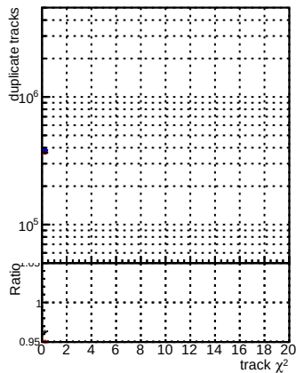
retrain
