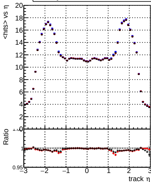
mean hits vs \eta — DQM_mkFit_TT_base — DQM_mkFit_TT_retrain_noCandDNN — DQM_mkFit_TT_retrain
