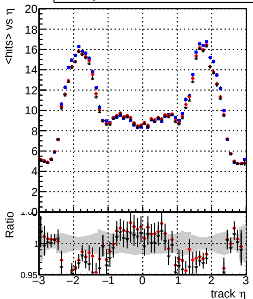
mean hits vs \eta — DQM_mkFit_TT_base — DQM_mkFit_TT_retrain_noCandDNN — DQM_mkFit_TT_retrain
