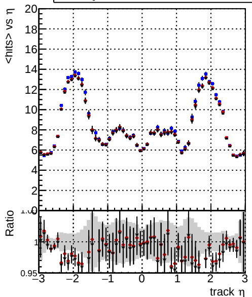
mean hit — DQM_mkFit_TT_base — DQM_mkFit_TT_retrain_noCandDNN — DQM_mkFit_TT_retrain
